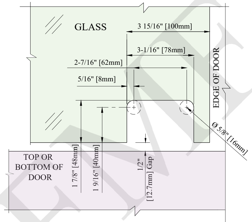
GLASS FABRICATION
