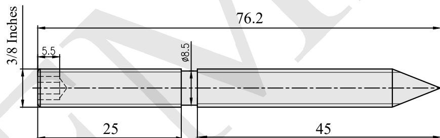
3 inches Length: SCS-03S
