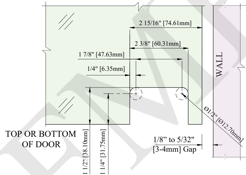
GLASS FABRICATION TEMPLATE
