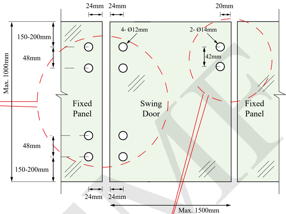
GLASS FABRICATION
