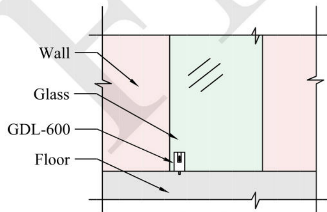
GDL-600 Floor Detail
