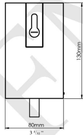
Elevation (Floor Mount)
