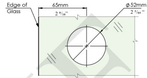
Glass Fabrication (Wall Mount)
