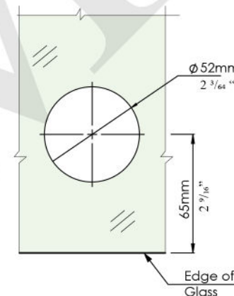
Glass Fabrication (Floor Mount)
