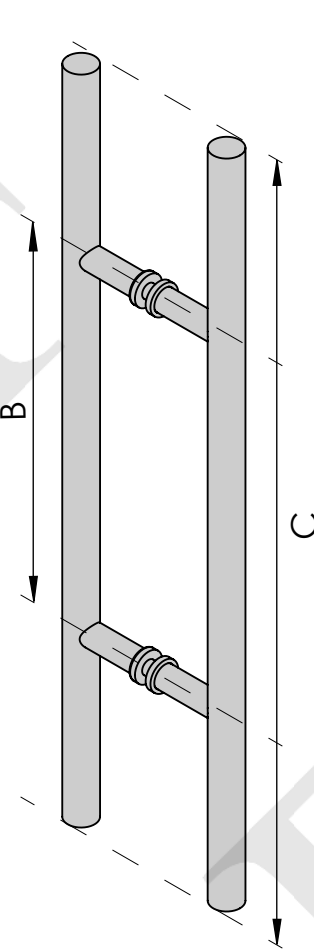
3D VIEW
