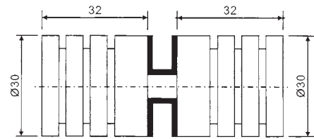
Dia: Ø25-Ø40
