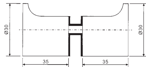
Dia: Ø25-Ø40
