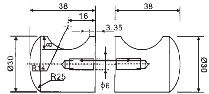
Dia: Ø25-Ø40
